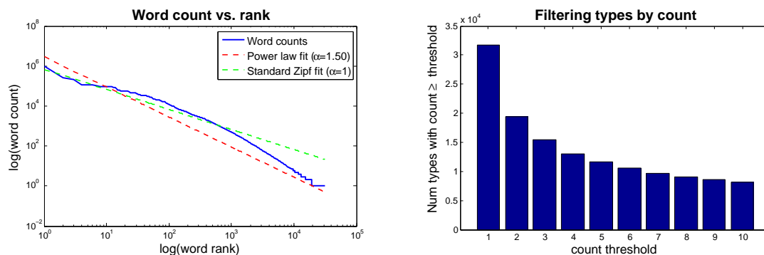
(a) Relationship between word frequency and word rank on a log-log plot, along with power laws with \alpha = 1 (Zipf's Law) and \alpha = 1.5 .
