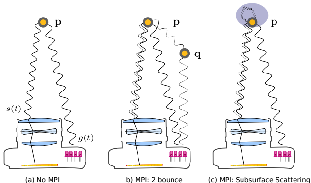
Figure 1. Multipath interference in time of flight cameras. In (a) the typical operation of TOF cameras is shown. A single optical path returns to the image sensor. In (b) an indirect bounce from point q to p causes two optical paths to return to the image sensor. In (c), subsurface scattering causes many optical paths to return to the sensor (one possible path is shown).
