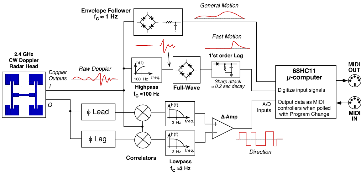
Figure 21: Signal conditioning for motion radar system
