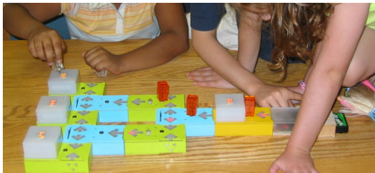
Figure 1: A “normal distribution” simulation
