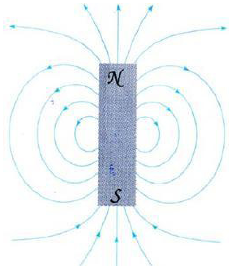
Magnetic field
