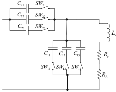
Fig. 7. The schematics of the adaptive L-match network.
