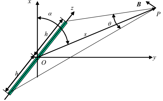
Fig. 3. Magnetic field generated by a dipole.
