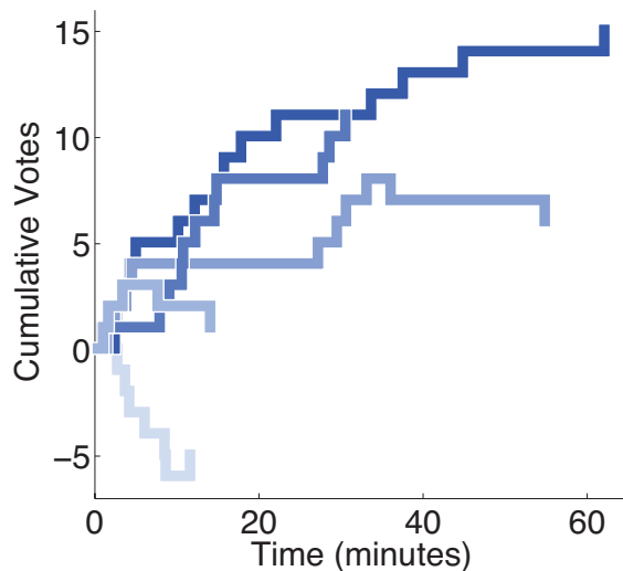
Figure 4 The evolution of the scores of posts over time, counting positive votes as +1 and negative votes as -1. Different colored lines are different posts.
