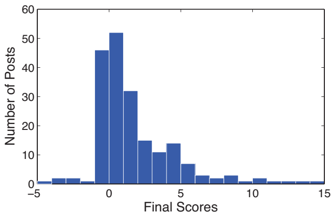
Figure 5 Distribution of final post scores, counting positive votes as +1 and negative votes as -1.
