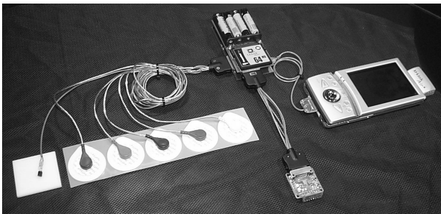
Figure 2: MITHril system, composed of the Zaurus PDA (right) with sensor hub and physiological sensing board (top), EKG/EMG/GSR/ temperature electrodes and sensors (left) and combined three-axis accelerometer and IR tag reader (bottom)
