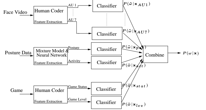
Figure 1: The overall architecture
