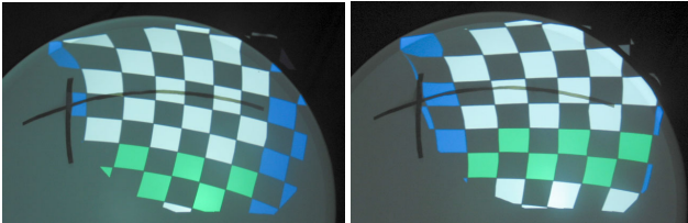
Figure 3: Left: uncorrected projection from a skew projector; Right: correction of the texture using constrained LSCM. Observe the change in the area at upper-left. Image is world horizontal aligned. Vertical stretch is minimized (at the cost of horizontal distortion) so that horizontal lines in the input texture remain in horizontal planes.
